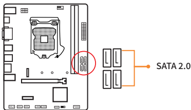
2-10 SATA Interface
