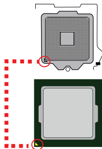
Figure 2-6 CPU installation
