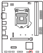
2-1 Clear CMOS Jumper CLR-CMOS
