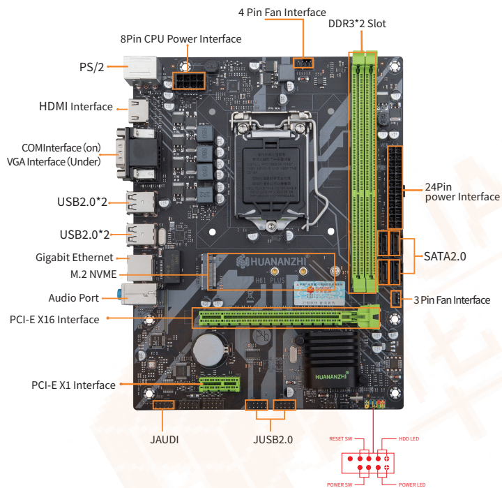
1-1 H61 PLUS MotherBoard Illustration
